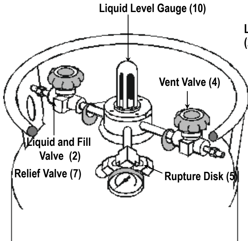
Low Pressure Design
