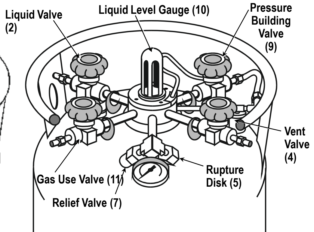
High Pressure Design
